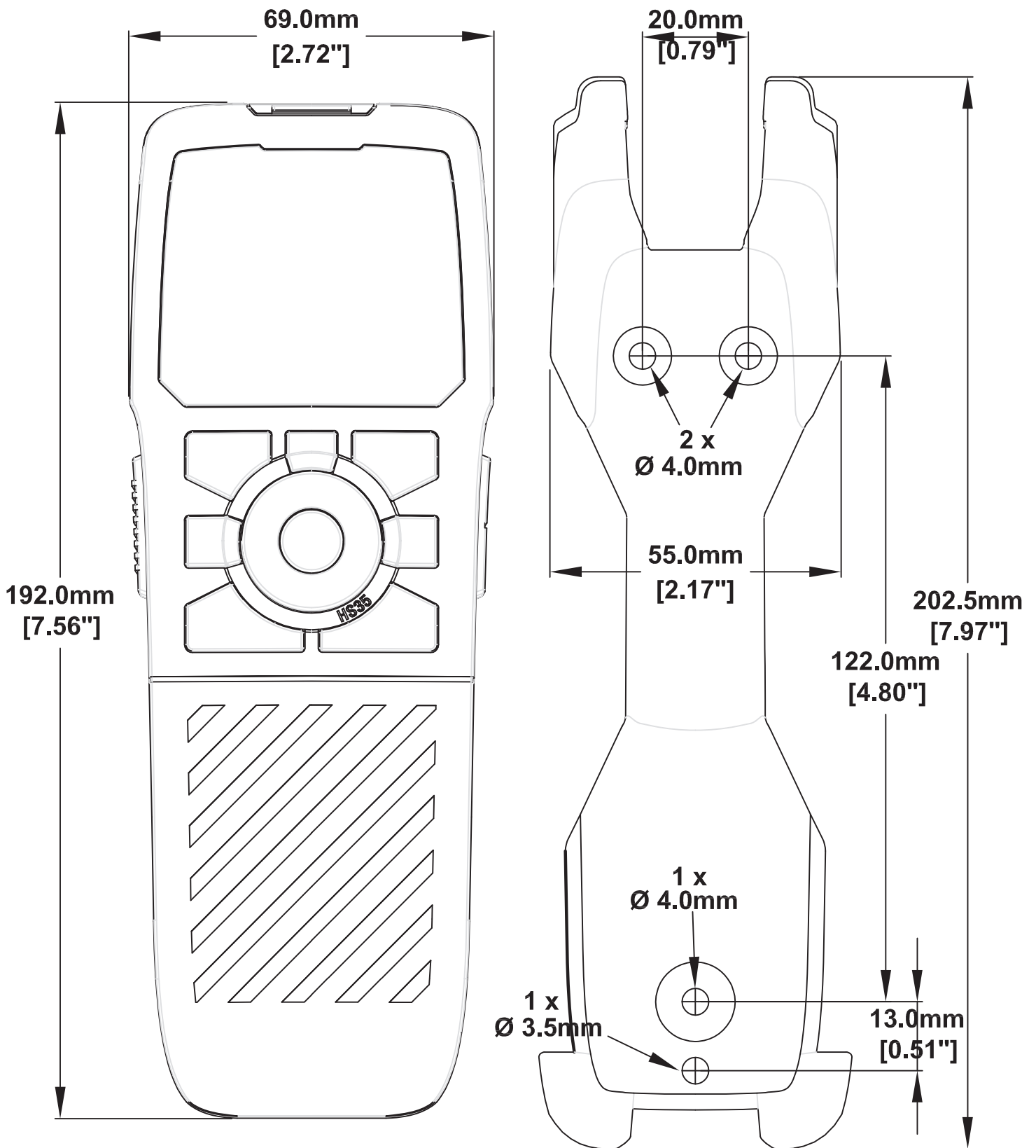
HS35 MOUNTING TEMPLATE SCALE 1:1 (Type-D)
